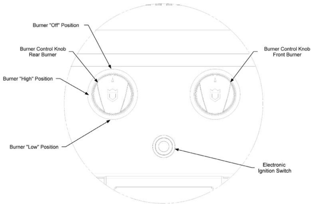
FIGURE 12B. VALVE POSITIONS SIDE BURNER WITHOUT LIGHT PACKAGE
